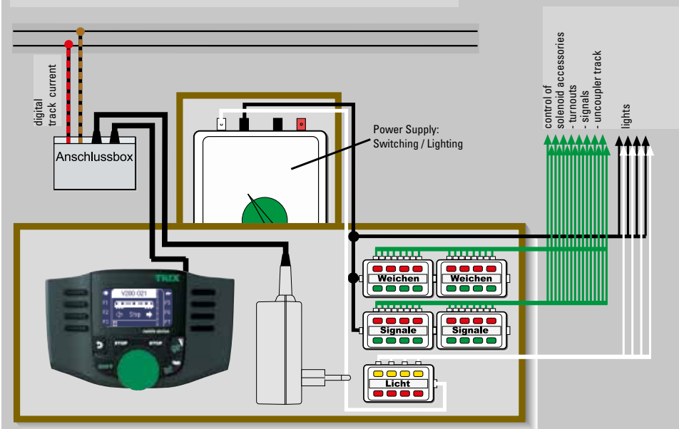
Running locomotives digitally with a Mobile Station and operating turnouts and signals with control boxes
