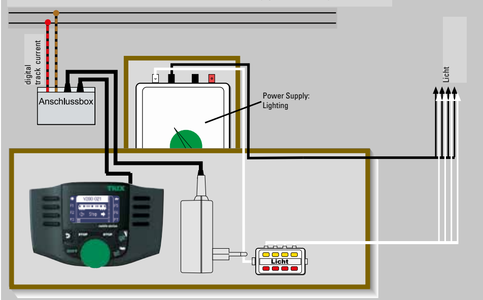
Running locomotives and operating turnouts and signals digitally with a Mobile Station and control boxes for controlling power to lights
