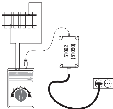
Connecting the switched mode power pack to the wall outlet
